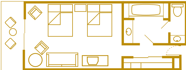
Typical Standard Room Parking & Landscaping View, with 1 king-size bed and 1 single day bed or 2 queens and 1 single day bed, 437 sq. ft. Accommodates up to five Guests plus one child under age 3 in a crib.
